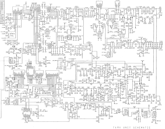
TXRX UNIT SCHEMATIC
