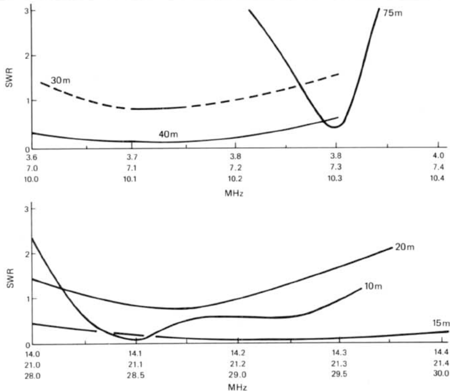
Fig. 9— S.w.r. curves for the six-band vertical.
